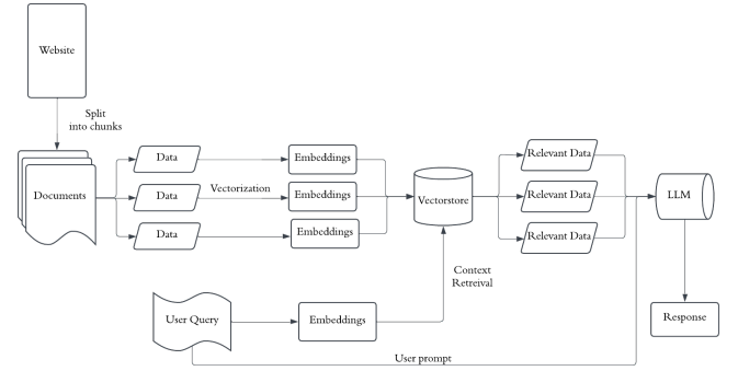
Figure 1: A depiction on how the RAG pipeline operates
